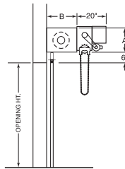
BELT DRIVE MOTOR
